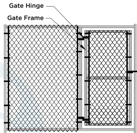
Gate Panel Elevation
