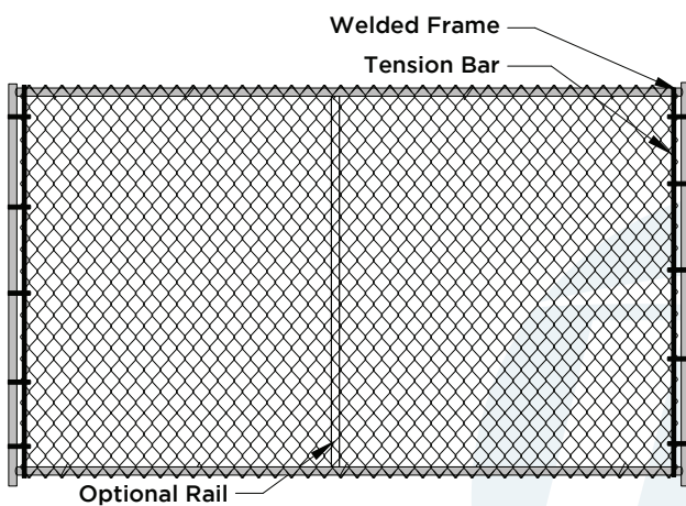
Side and Back Panel Elevation
